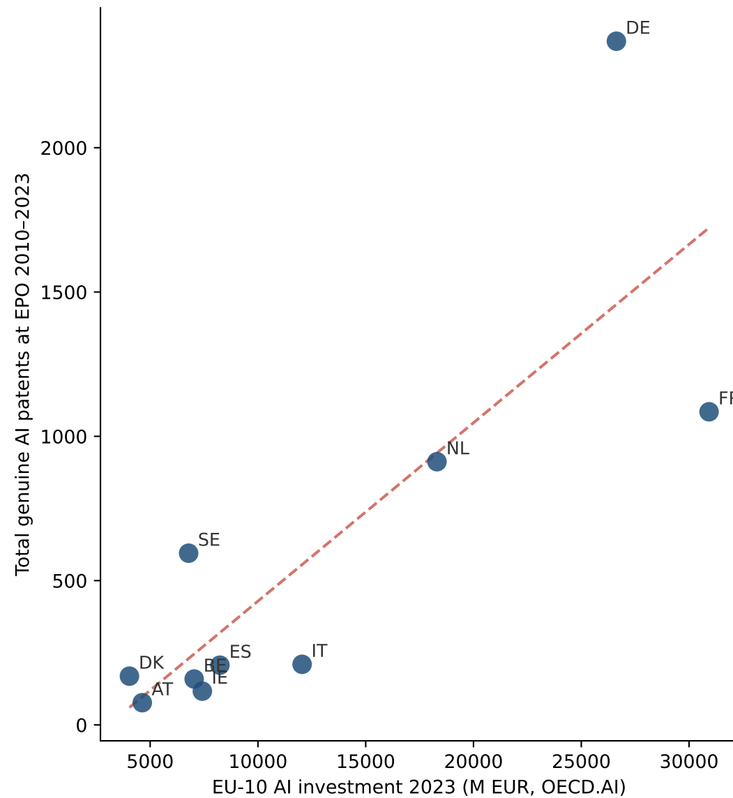
(b) EU-10: investment vs EPO patenting ( r = 0.82 )
